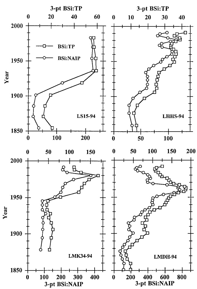
Fig. 14. Biogenic silica:total phosphorus (BSi:TP) and biogenic silica:nonapatite inorganic phosphorus (BSi:NAIP) versus date in Lake Superior, Lake Huron, and Lake Michigan sediment cores.
