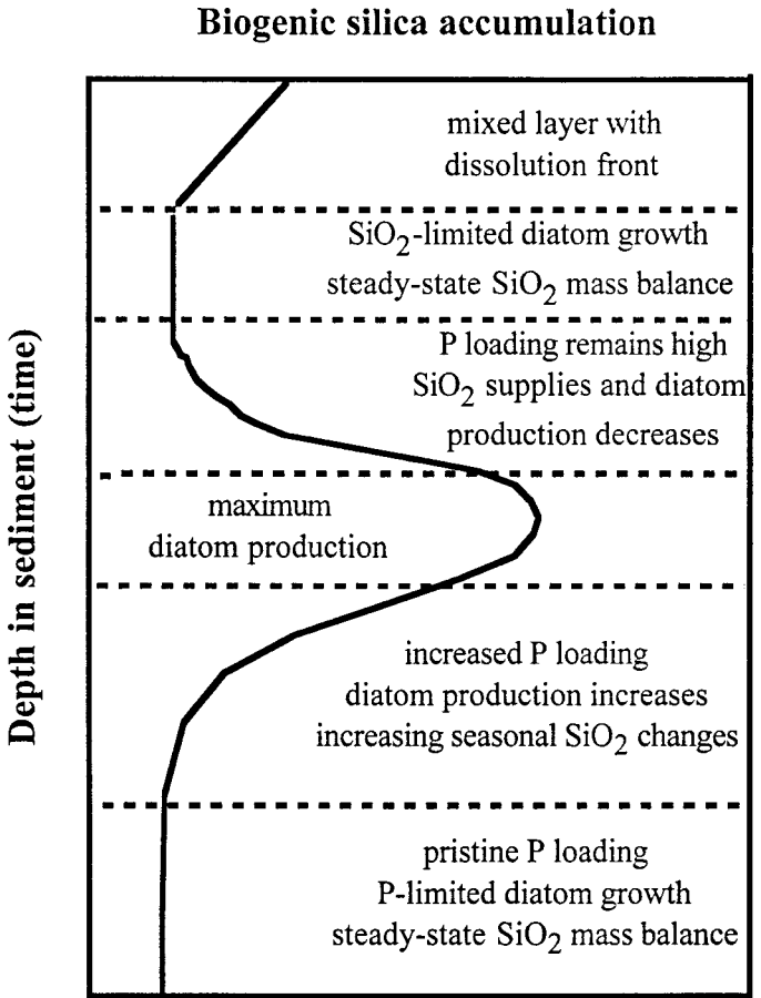
Fig. 2. Hypothetical model of BSi accumulation in the sediment record (from Schelske et al. 1983).
