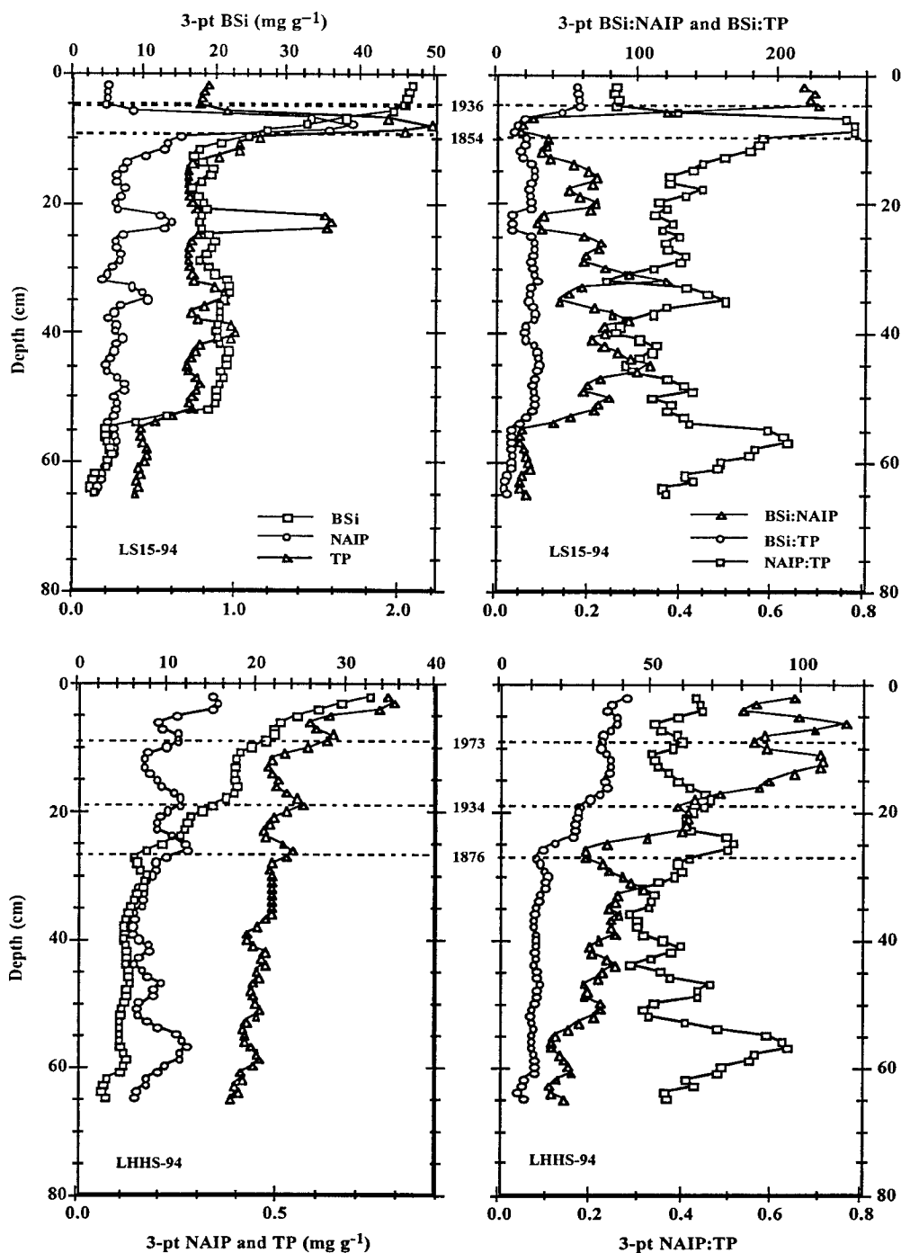
Fig. 4. Depth profiles of biogenic silica (BSi), total phosphorus (TP), and nonapatite inorganic phosphorus (NAIP) and their stoichiometry in sediment cores from Lake Superior and Lake Huron.
