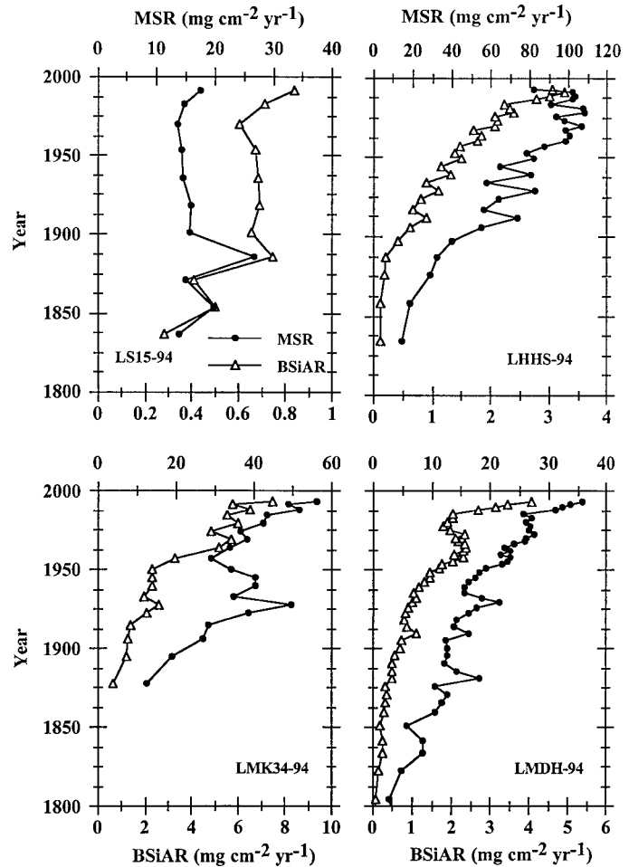
Fig. 12. Mass sedimentation rate (MSR) and biogenic silica accumulation rate (BSiAR) versus date for Lake Superior, Lake Huron, and Lake Michigan sediment cores.
