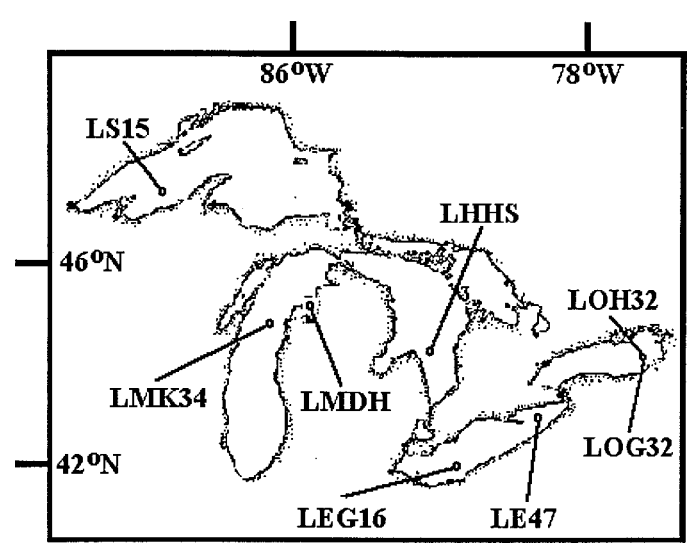
Fig. 1. Map with coring stations in the Great Lakes. Cores are identified with an alpha numeric code. The first two letters are codes for the lake; these codes are followed by station identification. In the text, the two numbers following the hyphen represent year of collection.
