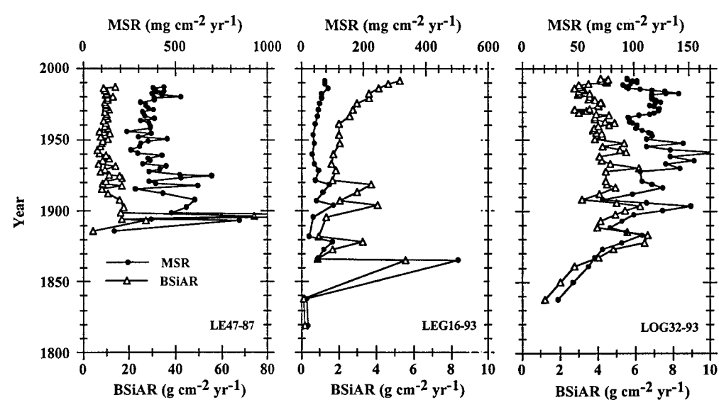
Fig. 13. Mass sedimentation rate (MSR) and biogenic silica accumulation rate (BSiAR) versus date for Lake Erie and Lake Ontario sediment cores.
